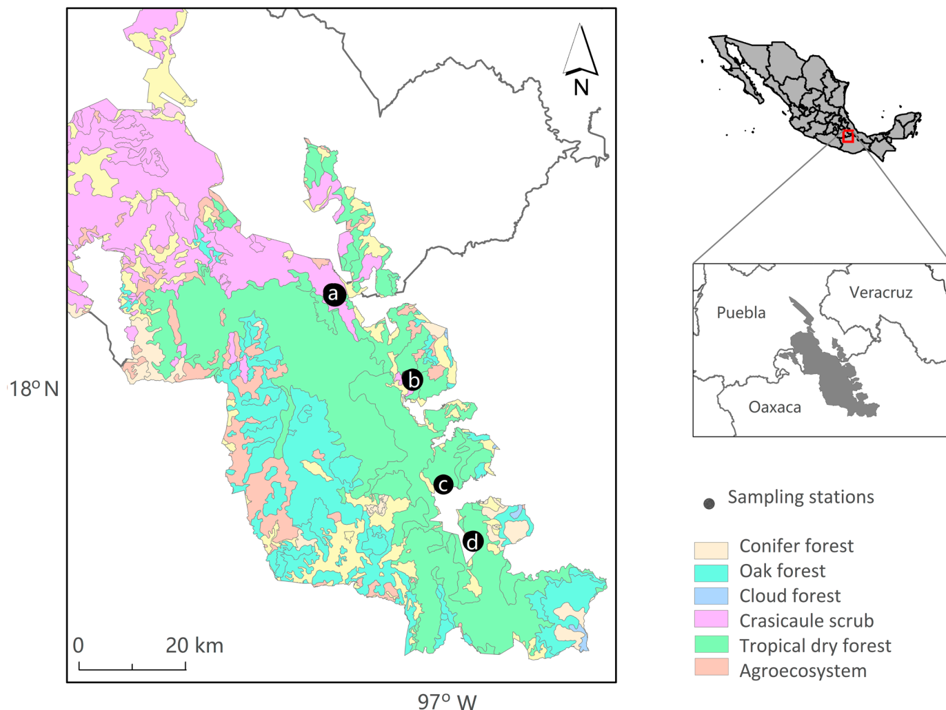
Figure 1. Geographical localization of the Tehuacán-Cuicatlán Biosphere Reserve, the main types of vegetation, and the location of four localities Casa Blanca (A), Los Cues (B), Cuicatlán (C), and Chcozapotes (D) in the region of La Cañada, Oaxaca.
